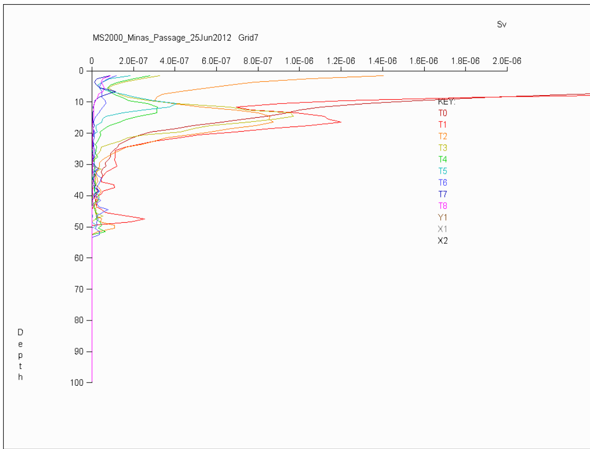
Relative S_v (linear) vs. depth (m) Grid 7, 25 June 2012 Minas Passage survey. Intensive grid lines T0 – T8 only.
