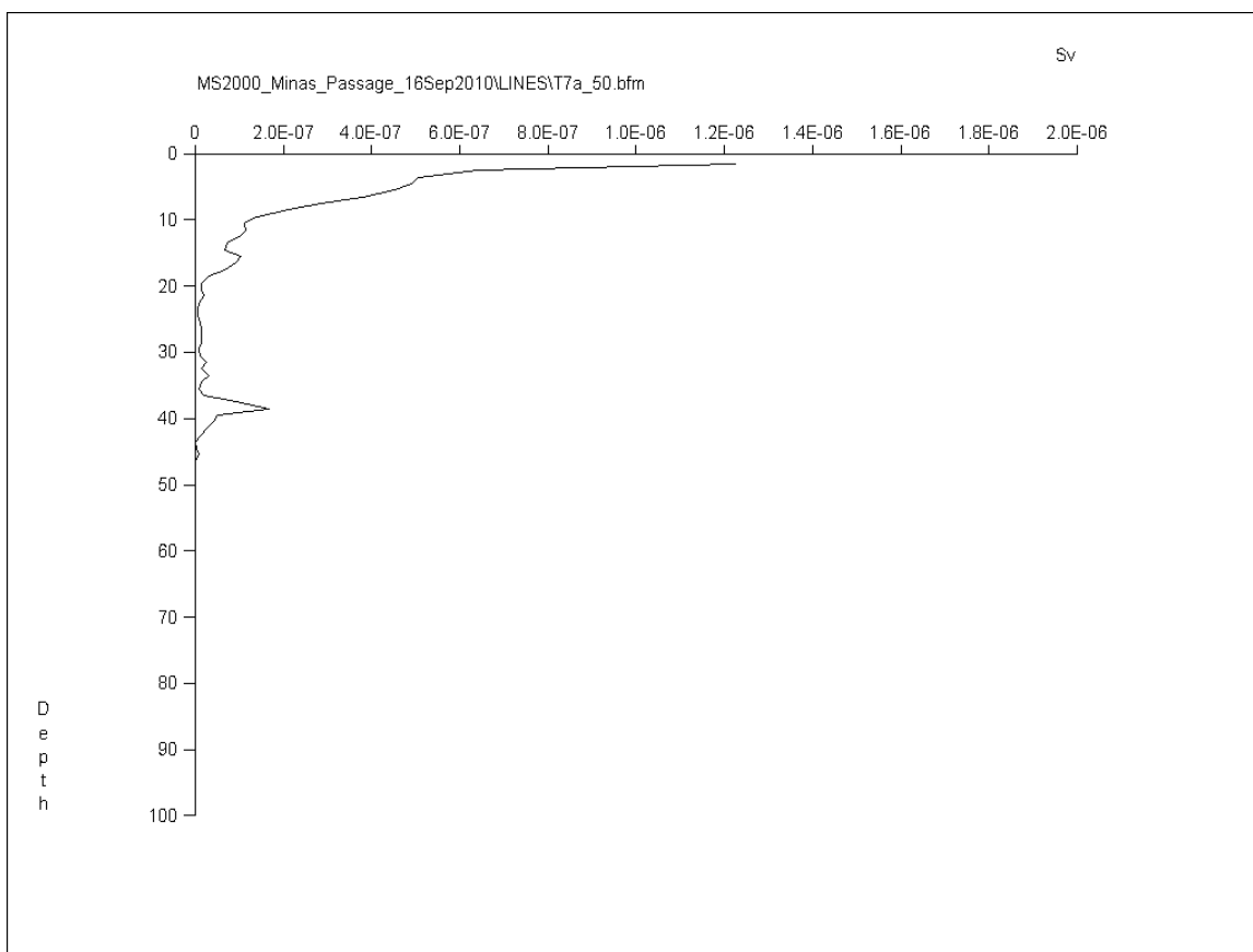
16 Sept. 2010. From 11:13:16 – 11:17:54 ADT. Line T7a. Recorded on declining ebb tidal flow.
