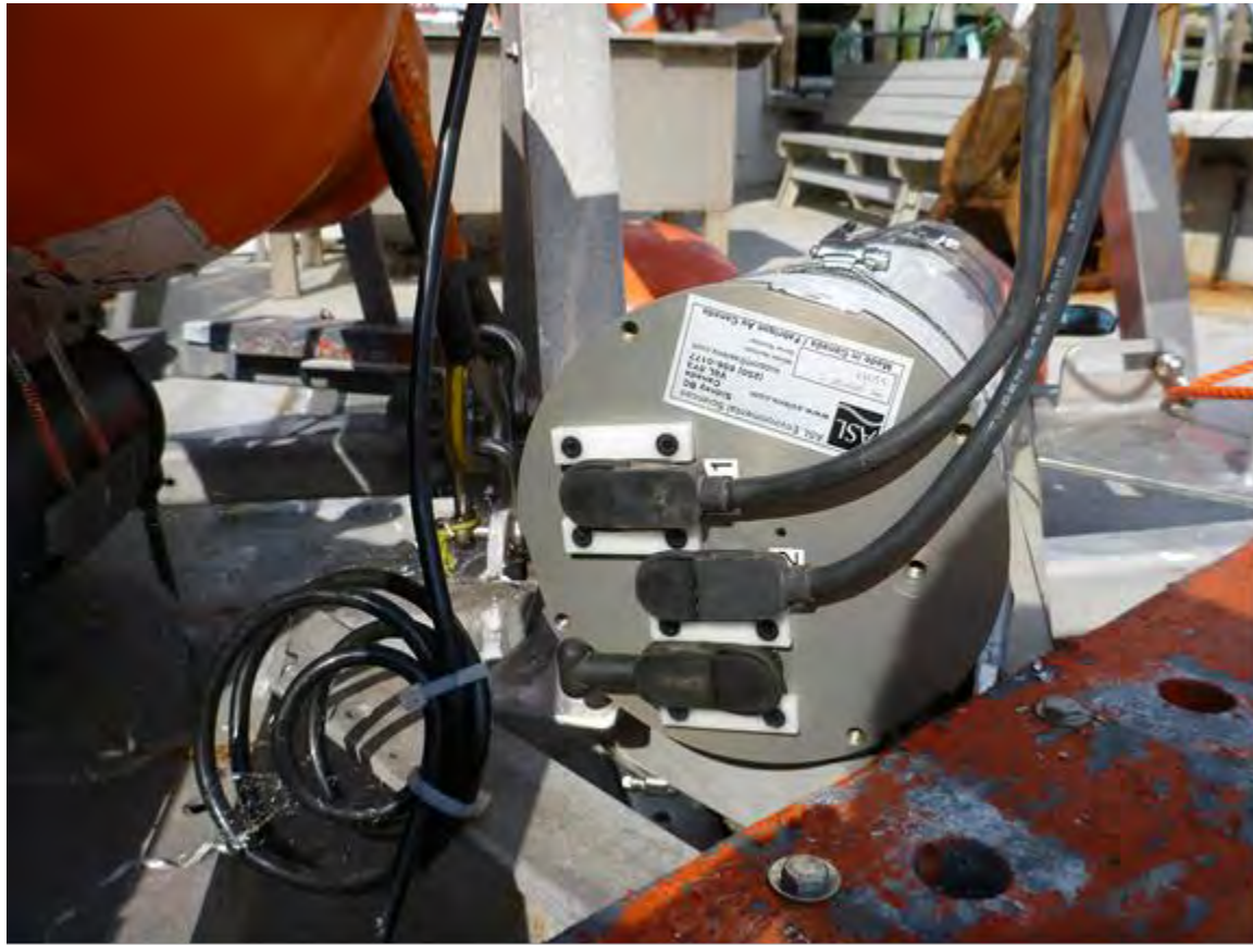
Figure A4-3. Close-up of the ASL water column profiler illustrating the communication port and the transducer connecting cables.
