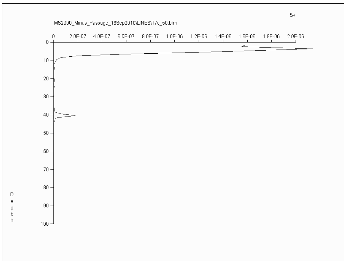
16 Sept. 2010. From 13:37:03 – 13:49:07 ADT. Line T7c. Recorded around LT slack water (13:38 ADT).
