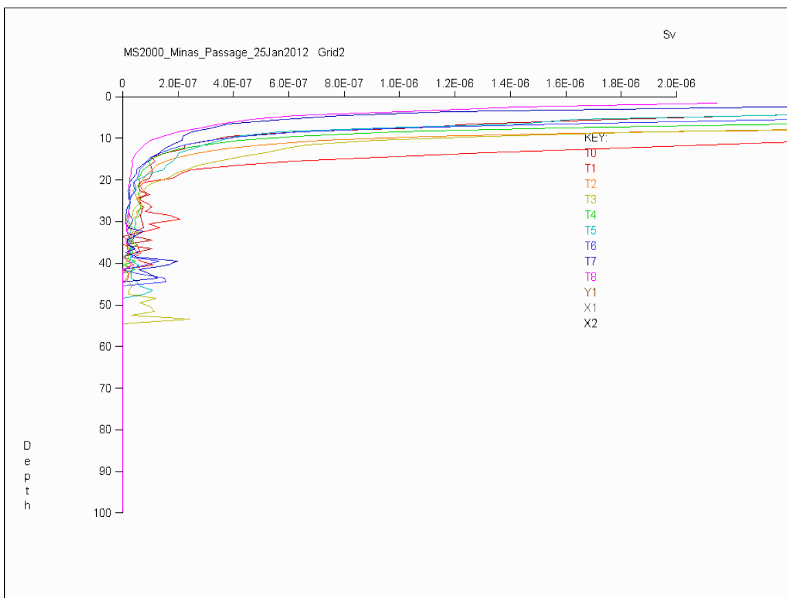
Relative S_v (linear) vs. depth (m) Grid 2, 25 Jan. 2012 Minas Passage survey. Intensive grid lines T0 – T8 only.
