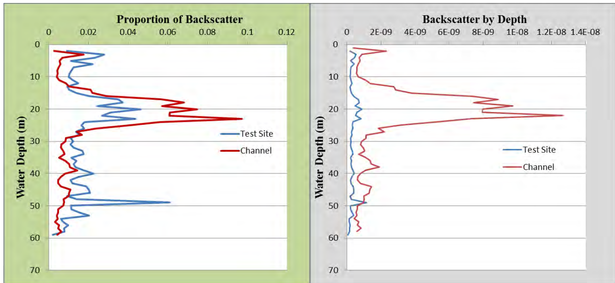
Figure 12a. Summary of the proportion (left) and actual (right) backscatter on September 19, 2011 for the test area and the channel to the test site water depths.
