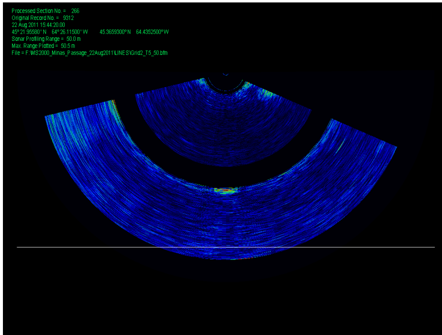
Figure A7-3. MS 2000 multi-beam fan sections without and with noise reduction:
