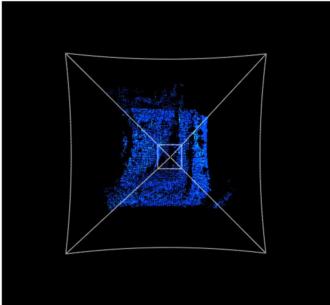
Figure A3-5. Coda sonar playback frame with colour-coded signal intensity from Eastern Wolf Island, Passamaquoddy Bay fish weir. Sonar is just below surface pointed downward about 25^{\circ} from the vertical and looking into the weir enclosure. Eye and sonar position are at the cross-hairs. Vertical structures on right of image and extending into the distance arise from a series of weir poles defining the RHS of the inner weir enclosure. The level bottom is at the bottom of the frame. Left of center is a mass of herring extending down from the surface in bowl-shaped wall. LHS of herring mass lies outside sonar's 50 \times 50^{\circ} total field of view.
