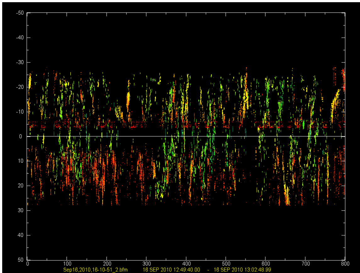
Figure 27. Aerial view of observed Simrad MS 2000 multi-beam field of view, looking downwards, over pings 1 to 800 of beamformed file Sept16,2010,16-10-51_2.bfm. Data series extends from 12:49:40 to 13:02:49 GMT, 16 Sept. 2010. This recording was conducted while the vessel steamed a loop just east of the turbine when shallow fish targets were especially numerous on the strong ebb tide cycle. Data are reproduced out to a maximum radial range of 28 m from the transducer. Negative to positive Y axis values correspond to Port and Starboard distances respectively from the transducer in meters. The X axis shows ping number. Depth is colour-encoded, ranging from red at surface to blue at depth. Shallow bubble clouds show up as shades of red to yellow while fish near 15 m depth appear in green. A few deeper fish targets or acoustic artefacts show up as blue.
