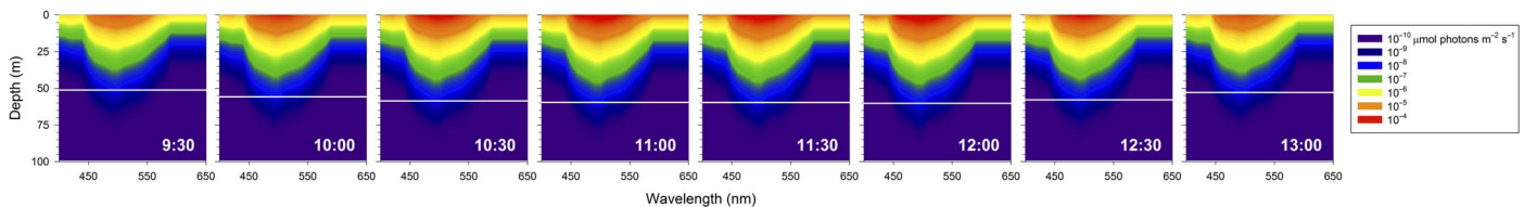
Fig. 3. Modeled depth of a constant light level (isolume) set to be the depth limit of copepod light-mediated behavior in Kongsfjorden. Underwater spectral scalar irradiance [ E_s(\lambda) , \mu\text{mol photons m}^{-2} \text{s}^{-1} ] was weighted by the spectral response of C. finmarchicus to yield a photometric quantity of Calanus -utilized light that is shown in colored contours as a function of depth at 30-min intervals on the 23 January Jetyak deployment. White horizontal lines show the depth of an isolume at 5 \times 10^{-8} \mu\text{mol photons m}^{-2} \text{s}^{-1} of Calanus -utilized light. UTC, coordinated universal time.
